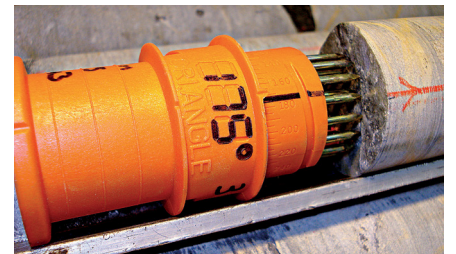
The REFLEX VERTI-ORI™ system in conjunction with the patented REFLEX ORI-BLOCK™ is a permanently auditable vertical core orientation method.
